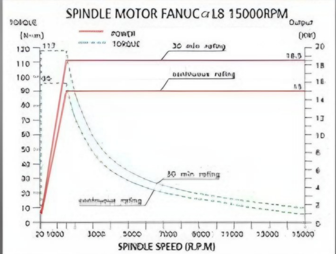
15,000/18,000 RPM DIRECT-DRIVE SPINDLE (OPTIONAL)
